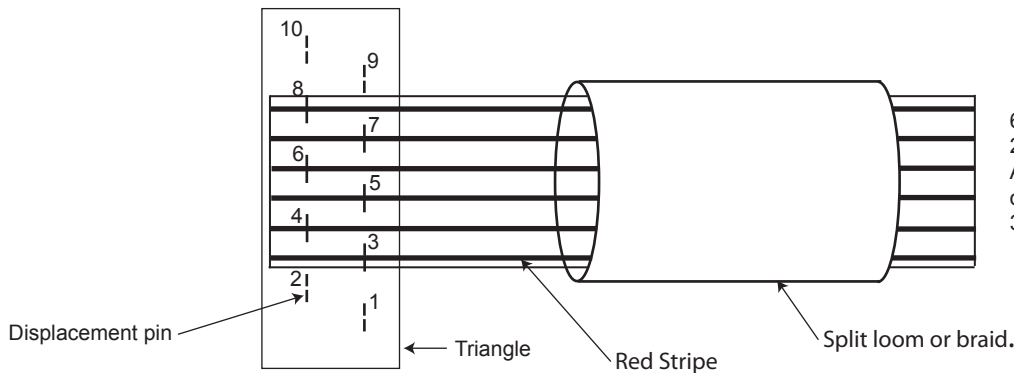
View from top of connector plug. Wires in displacement pins.
