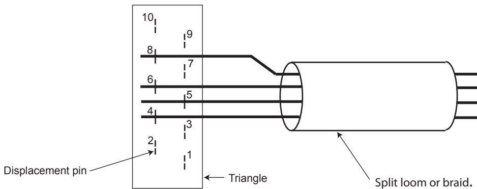
View from top of connector plug. Wires in displacement pins.
