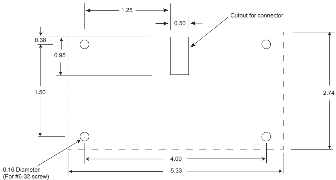
Mounting Cutout Template
